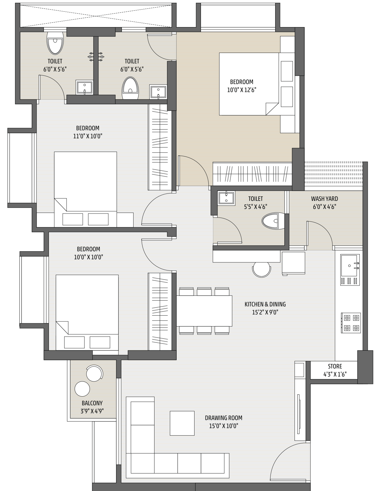
3 BHK UNIT PLAN
