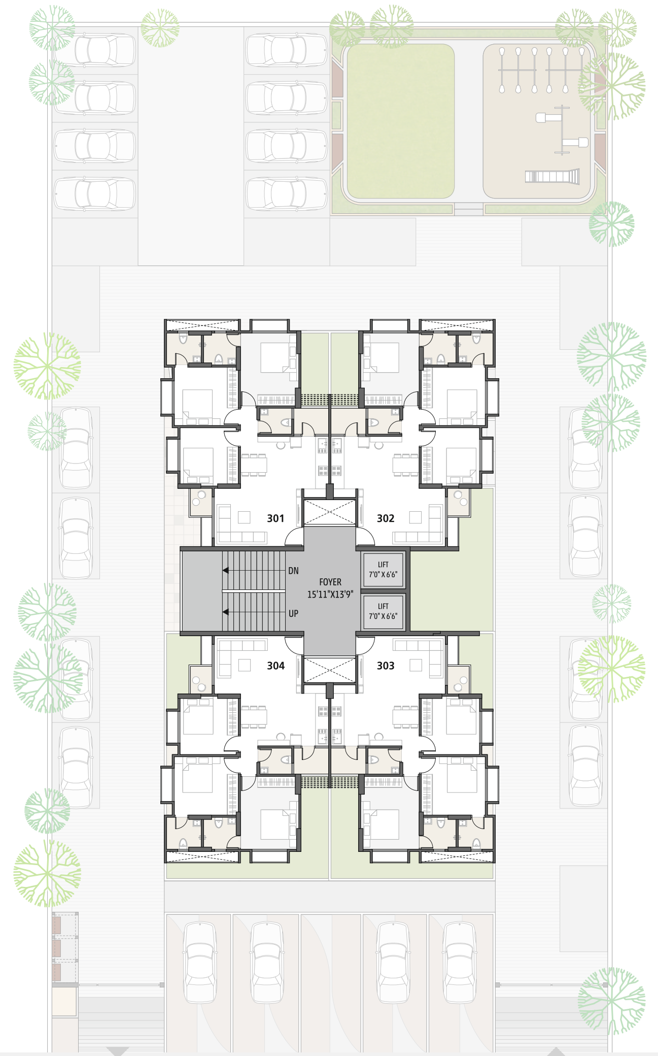
N TYPICAL FLOOR
